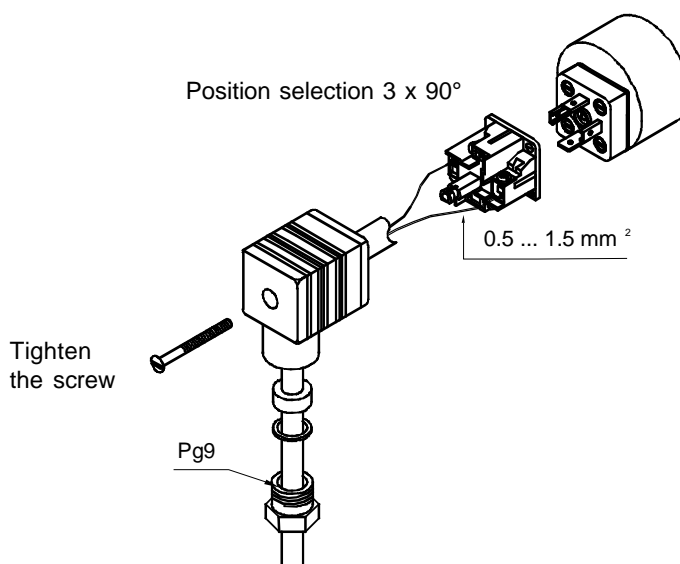
Figure 1-6 Adjusting the junction box position
