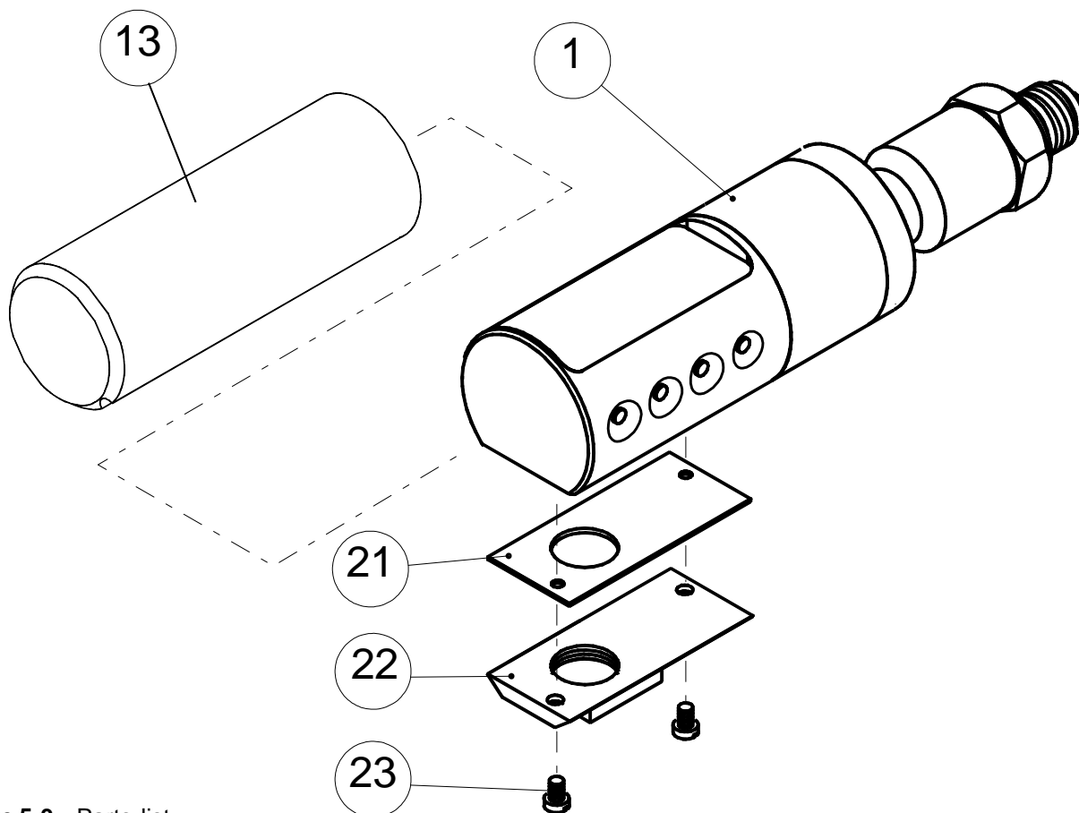
Figure 5-3 Parts list: Enclosure N, housing with display
