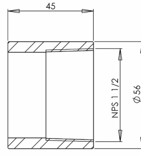
TA Coupling M1035224
