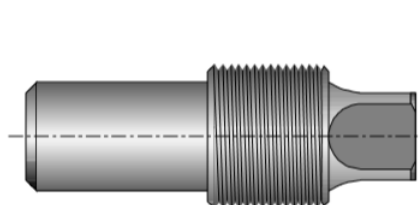
Welding assistant for Satron coupling G1, brass
