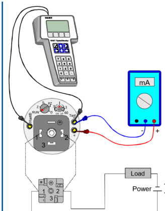
Housing with DIN43650 plug connector, housings H and T
