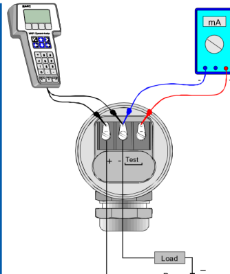
Housing with terminal strip, housing M
