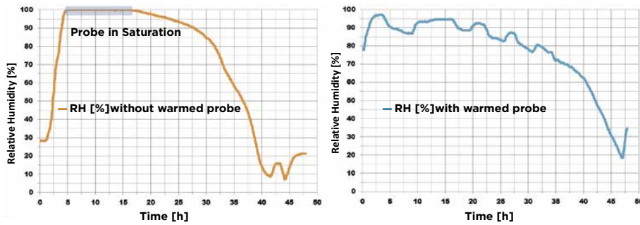
A 48-hour drying cycle with the old system (left) and the Vaisala HMT337 with warmed probe (right). The warmed-probe technology provides accurate relative humidity readings at the beginning of the process, where the non-heated probe is saturated by condensed water.
